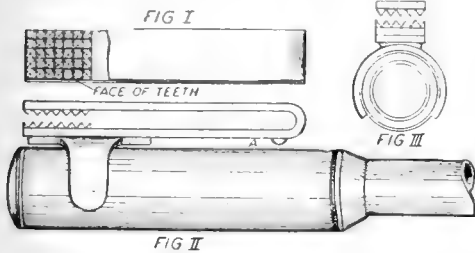
A check protector, a pen for writing the check, and a clip for holding the pen, all combined in one instrument
